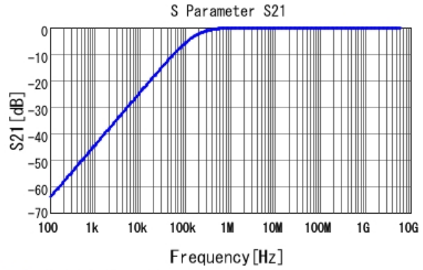
■ GRM033B10J103KA01 S21 DCOV, 20degC
