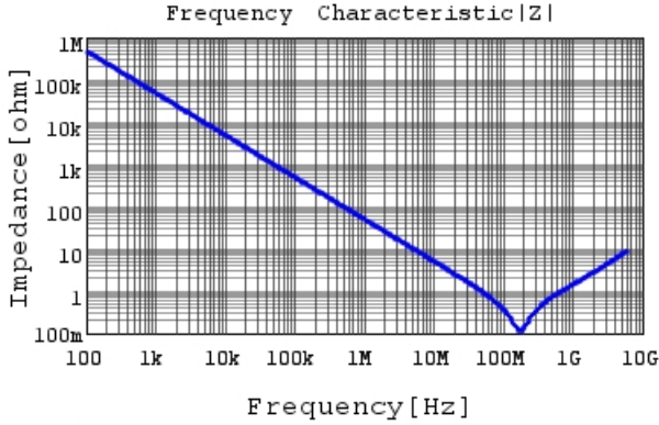
GRM033R71E332MA12 |Z| DCOV,25degC
