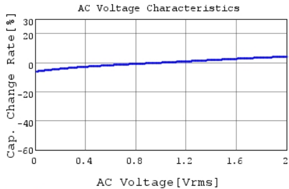
GRM033R71E332MA12 C-AC Voltage capchange, Dc
