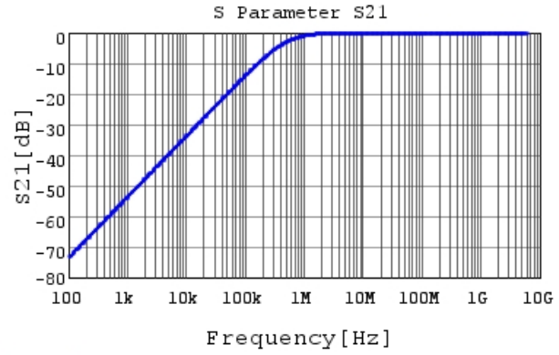
GRM033R71E332MA12 S21 DC0V,25degC
