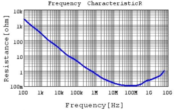
GRM033R71E332MA12 R DCOV,25degC
