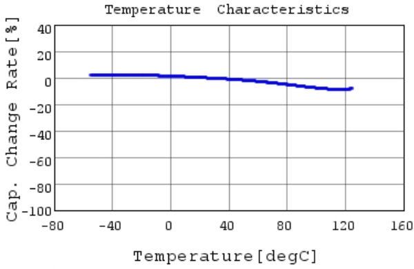
GRM033R71E332MA12 C-Temp. capchange, DC0.0V,
