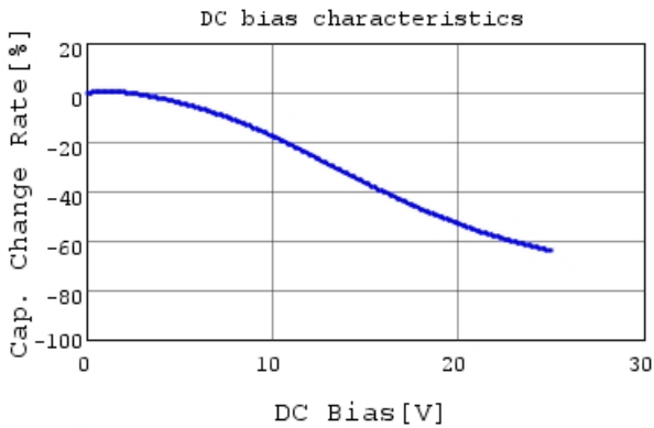
GRM033R71E332MA12 C-DC bias capchange, 25.0c
