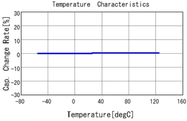
GRM0225C1C150JA03 C-Temp. capchange, DCOV, AC1Vrms
