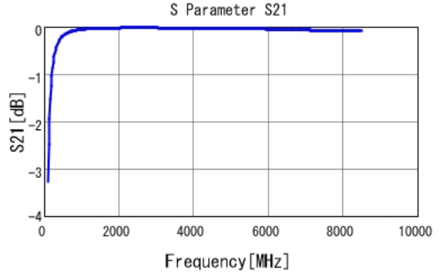
GRM0225C1C150JA03 S21 DCOV, 25degC
