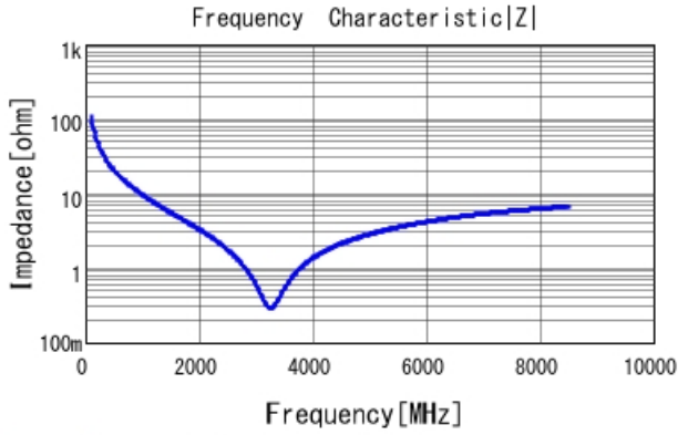
GRM0225C1C150JA03 |Z| DCOV, 25degC
