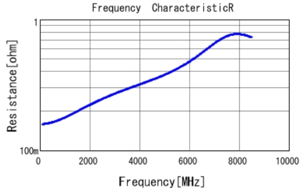
GRM0225C1C150JA03 R DCOV, 25degC
