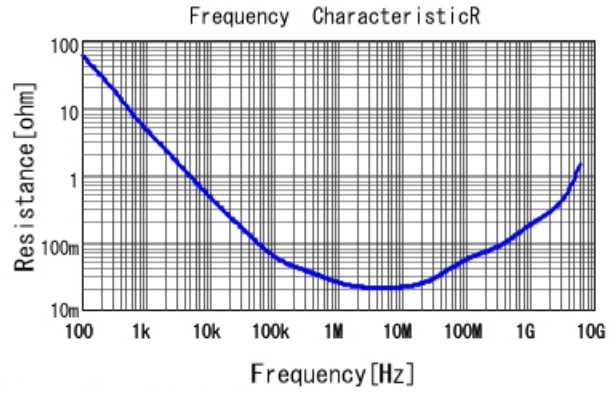
GRM152D70G224KE15 R DCOV, 25degC
