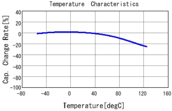
GRM152D70G224KE15 C-Temp. capchange, DC0.0V, AC0.5
