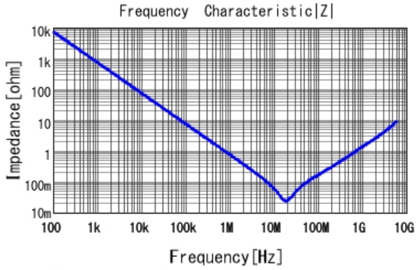
GRM152D70G224KE15 |Z| DCOV, 25degC
