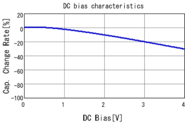
GRM152D70G224KE15 C-DC bias capchange, 25.0degC, A
