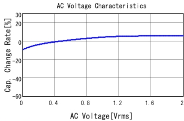
GRM152D70G224KE15 C-AC Voltage capchange, DCOV, 25
