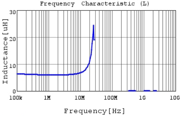
■ MDH7045C-6R8NB L
