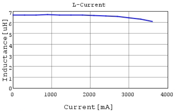
■ MDH7045C-6R8NB L-Current 20degC
