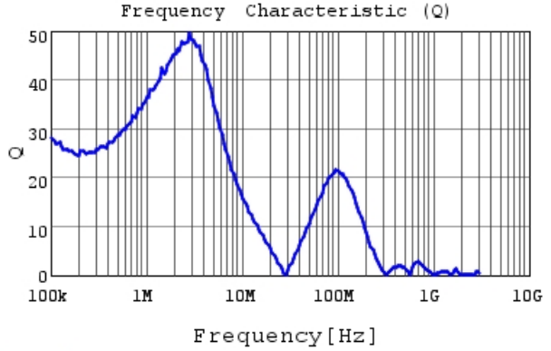
■ MDH7045C-6R8NB Q
