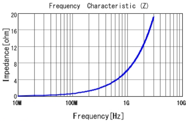
LQP03TQ1N0C02 |Z|
