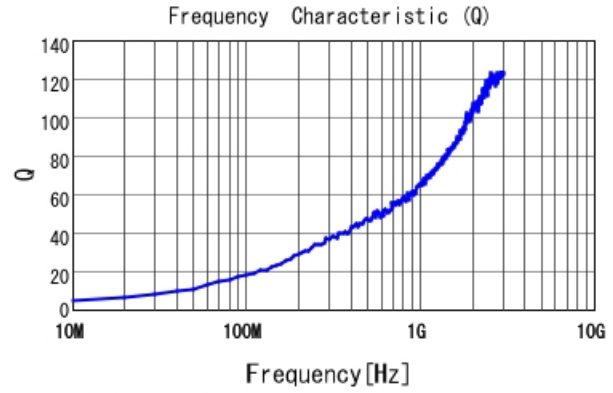
LQP03TQ1N0C02 Q
