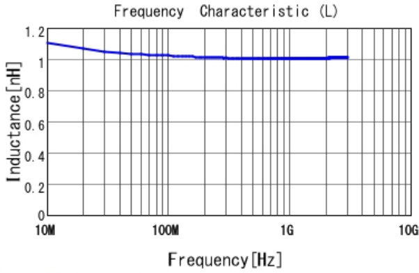
LQP03TQ1N0C02 L
