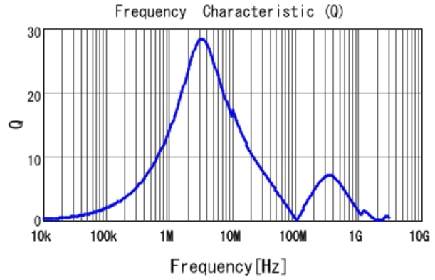
B1047AS-2R2N Q
