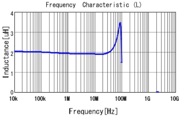
B1047AS-2R2N L
