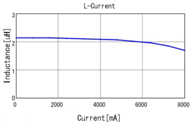
B1047AS-2R2N L-Current 20degC
