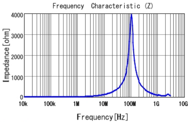
B1047AS-2R2N |Z|
