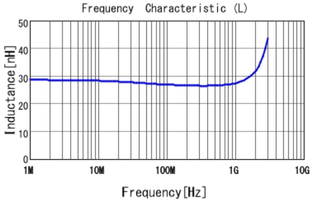
LQW15AN27NJ80 L
