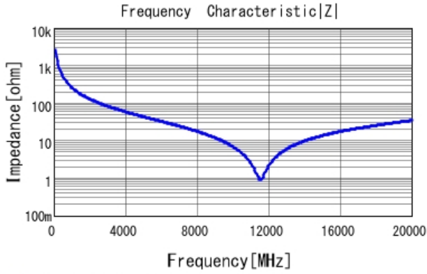
■ GRM0335C1HR60BA01 |Z| DCOV, 25degC
