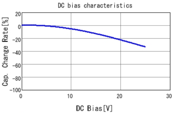
GRM188R71E154KA01 C-DC bias capchange, 25.0degC, A
