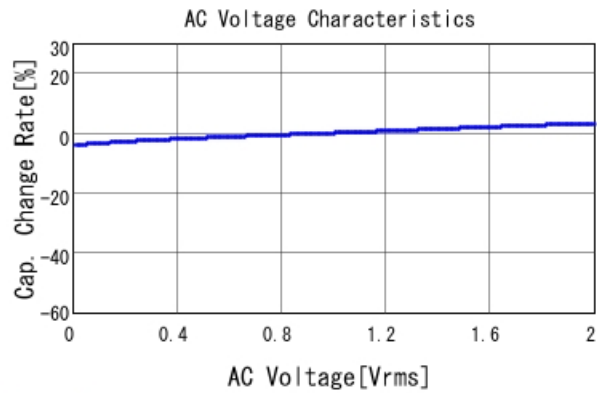
GRM188R71E154KA01 C-AC Voltage capchange, DCOV, 25
