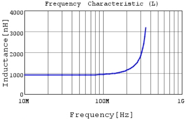
LQW2UASR91J0C L
