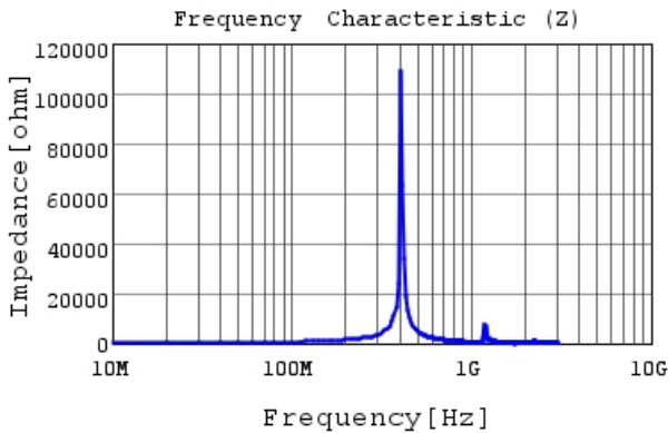
LQW2UASR91J0C |Z|
