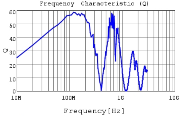
LQW2UASR91J0C Q
