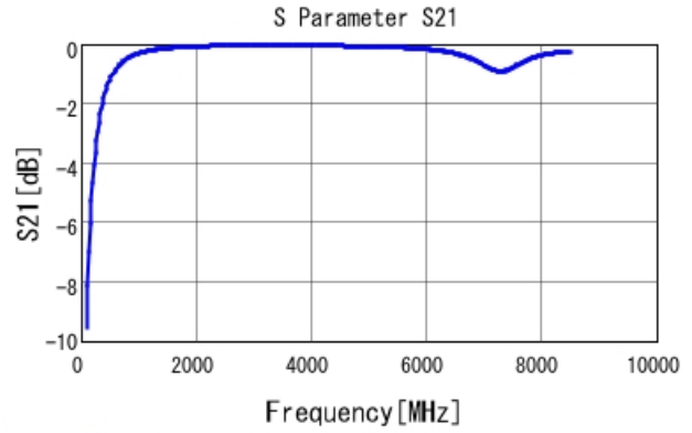
GRM1555C2A5R6DA01 S21 DCOV, 25degC
