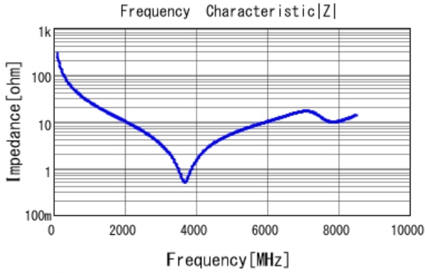
GRM1555C2A5R6DA01 |Z| DCOV, 25degC
