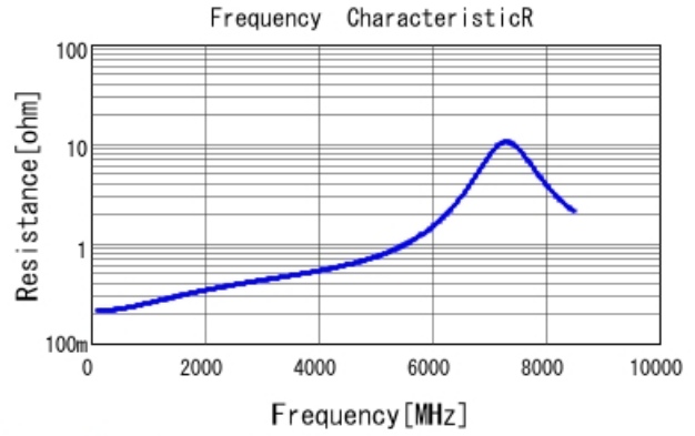
GRM1555C2A5R6DA01 R DCOV, 25degC
