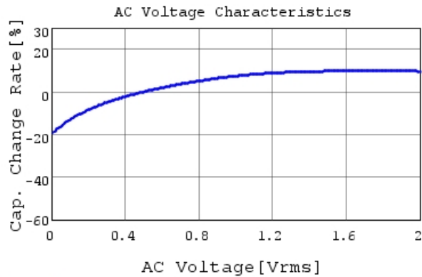
GRM033R61A393KE84 C-AC Voltage capchange, Dc
