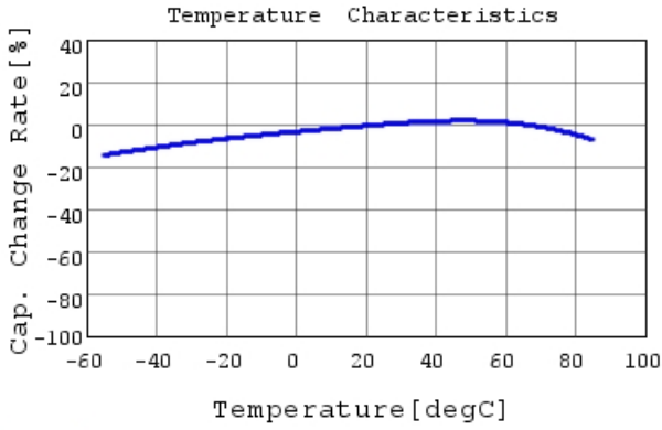
GRM033R61A393KE84 C-Temp. capchange, DC0.0V,
