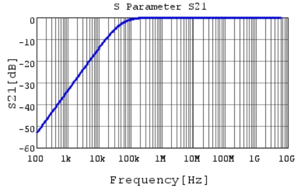
GRM033R61A393KE84 S21 DC0V, 25degC
