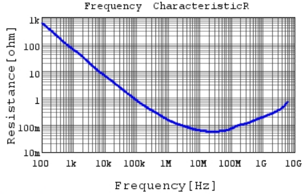
GRM033R61A393KE84 R DCOV, 25degC
