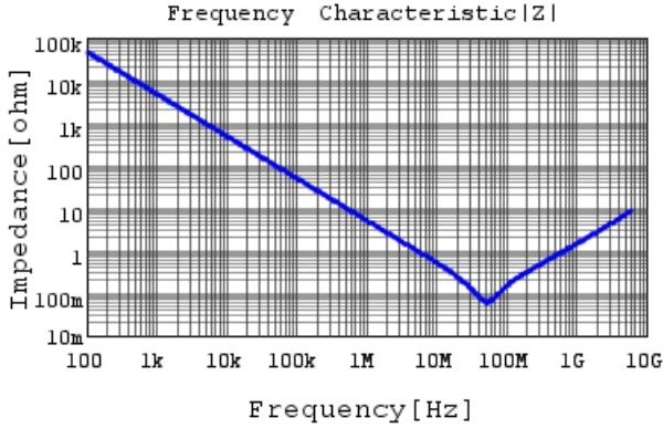
GRM033R61A393KE84 |Z| DCOV, 25degC
