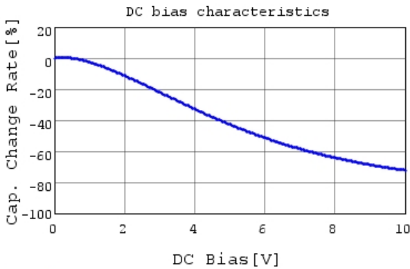
GRM033R61A393KE84 C-DC bias capchange, 25.0c
