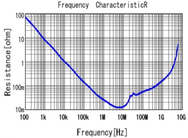
■ GRM188R71E474KA12 R DCOV, 25degC
