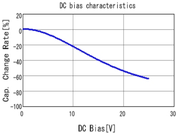
■ GRM188R71E474KA12 C-DC bias capchange, 25.0degC, AC1.
