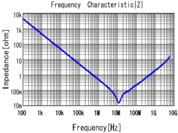
■ GRM188R71E474KA12 |Z| DCOV, 25degC
