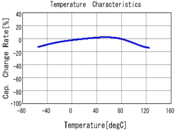
■ GRM188R71E474KA12 C-Temp. capchange, DCO. 0V, AC1.0V rm
