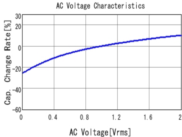
■ GRM188R71E474KA12 C-AC Voltage capchange, DCOV, 25.0d
