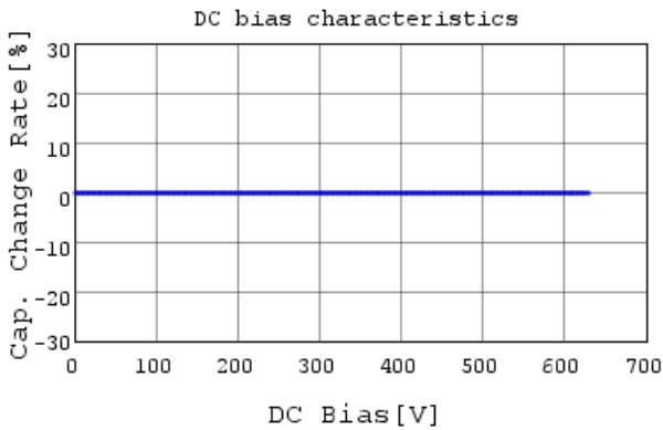
GRM31B5C2J681JW01 C-DC bias capchange, 25.0c
