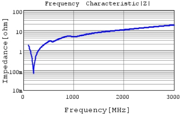
GRM31B5C2J681JW01 |Z| DC0V, 25degC
