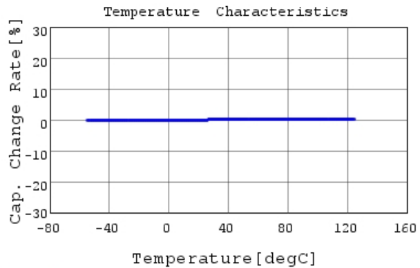
GRM31B5C2J681JW01 C-Temp. capchange, DC0V, 1
