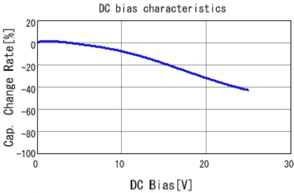
GRM155R71E123KA61 C-DC bias capchange, 25.0degC, A
