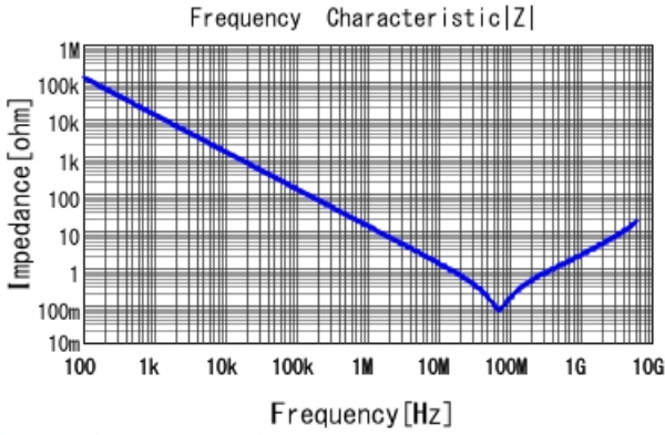
GRM155R71E123KA61 |Z| DCOV, 25degC
