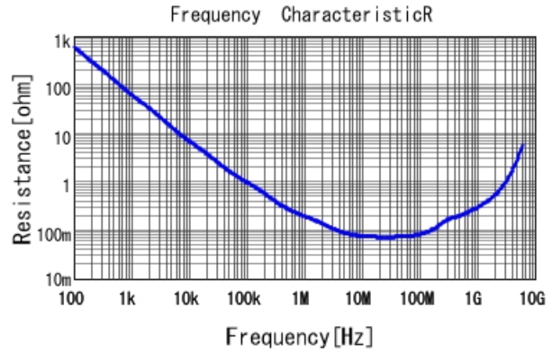
GRM155R71E123KA61 R DCOV, 25degC
