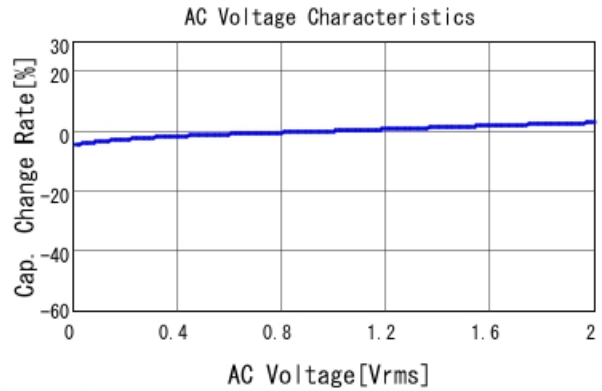
GRM155R71E123KA61 C-AC Voltage capchange, DCOV, 25
