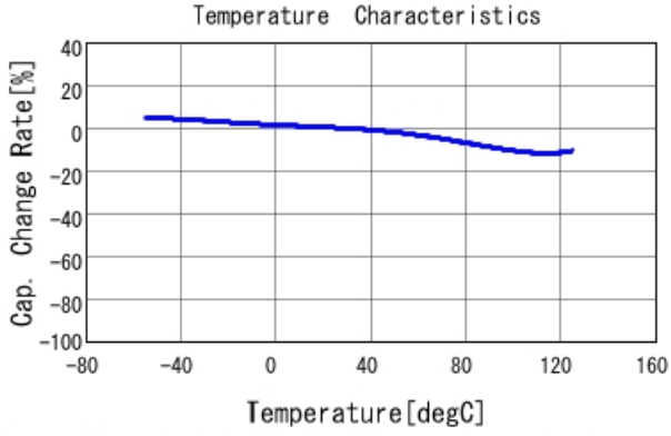
GRM155R71E123KA61 C-Temp. capchange, DC0.0V, AC1.C
