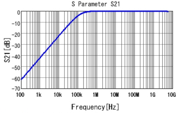
GRM155R71E123KA61 S21 DC0V, 25degC
