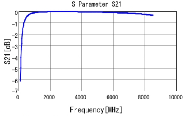
GRM0335C1H9R0CA01 S21 DCOV, 25degC
