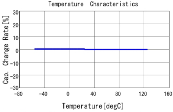
GRM0335C1H9R0CA01 C-Temp. capchange, DCOV, AC1Vrms
