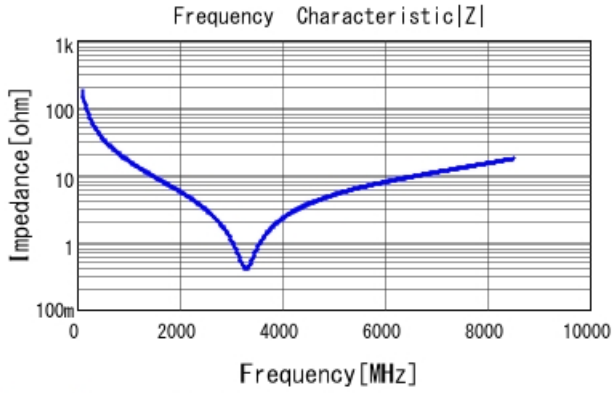
GRM0335C1H9R0CA01 |Z| DCOV, 25degC
