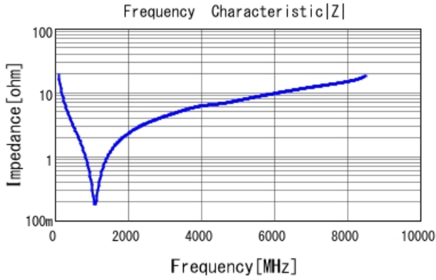
■ GRM0335C2A820JA01 |Z| DC0V, 25degC
