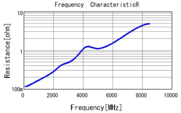
■ GRM0335C2A820JA01 R DC0V, 25degC
