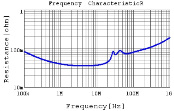
RCER71H224K1K1H03B R DCOV, 25degC
