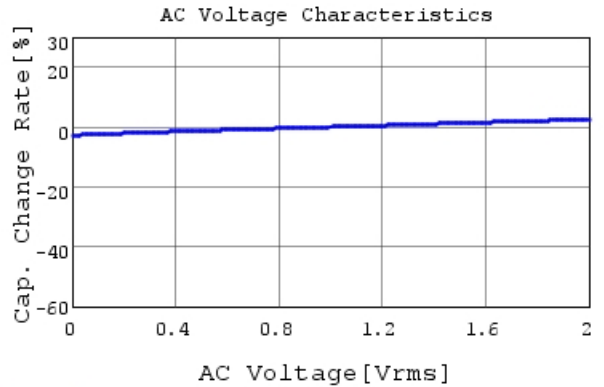
RCER71H224K1K1H03B C-AC Voltage capchange, I
