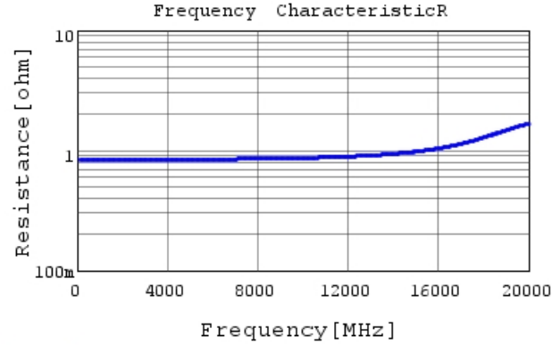
GRM0335C2AR70BA01 R DCOV, 25degC
