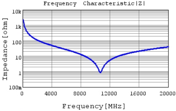
GRM0335C2AR70BA01 |Z| DCOV, 25degC
