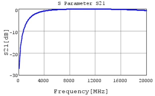
GRM0335C2AR70BA01 S21 DCOV, 25degC
