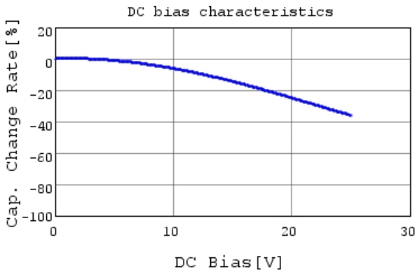
GRM033B11E152MA01 C-DC bias capchange, 20.0c
