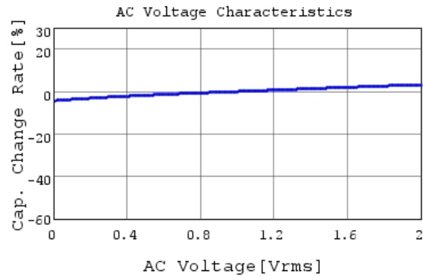
GRM033B11E152MA01 C-AC Voltage capchange, Dc
