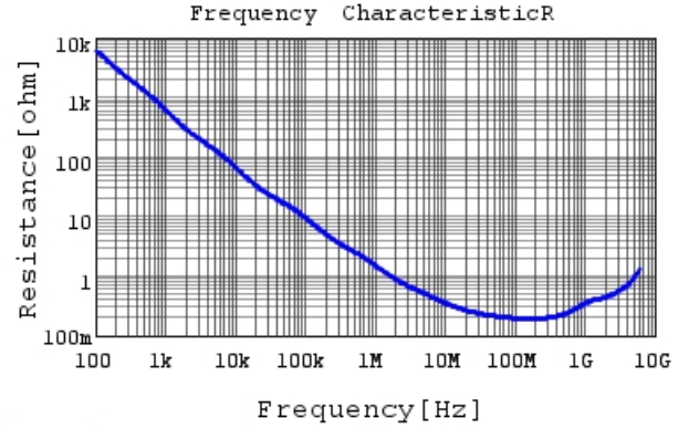
GRM033B11E152MA01 R DCOV, 20degC
