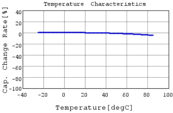
GRM033B11E152MA01 C-Temp. capchange, DC0.0V,
