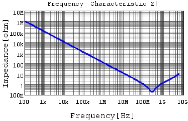
GRM033B11E152MA01 |Z| DCOV, 20degC
