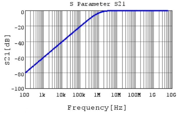
GRM033B11E152MA01 S21 DC0V, 20degC
