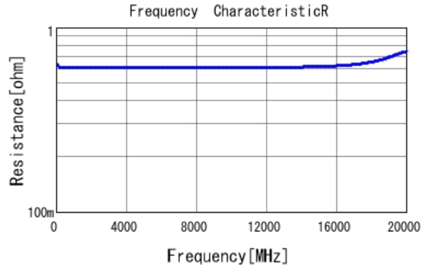
GQM1555C2DR10BB01 R DCOV, 25degC
