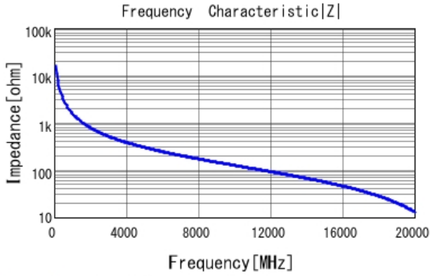
GQM1555C2DR10BB01 |Z| DCOV, 25degC
