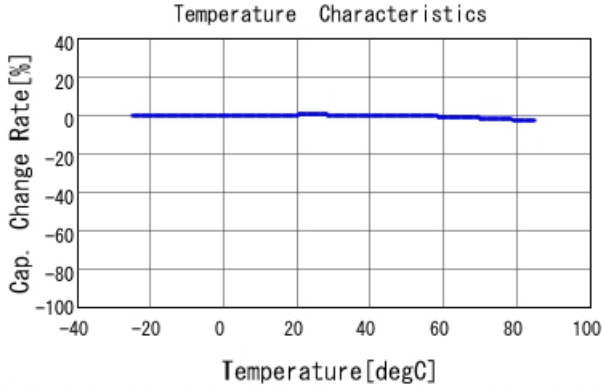
■ GRM033B31H151MA12 C-Temp. capchange, DCO. 0V, AC1. 0Vrm
