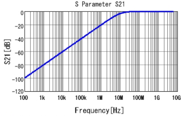
■ GRM033B31H151MA12 S21 DCOV, 20degC
