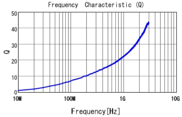
LQP02TQ2N2C02 Q
