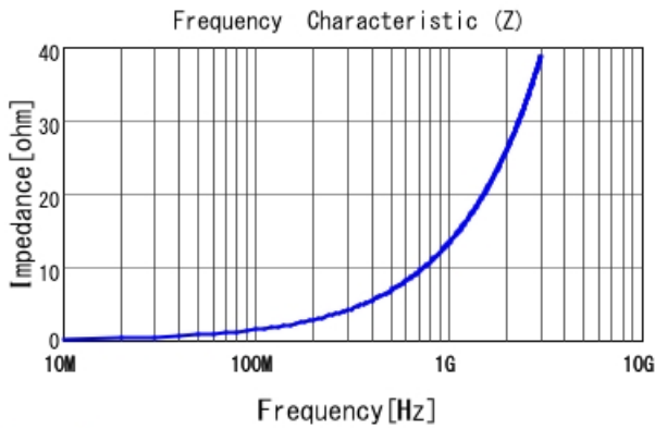
LQP02TQ2N2C02 |Z|
