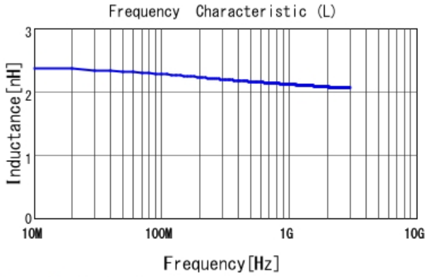
LQP02TQ2N2C02 L
