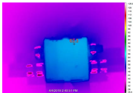
Figure 11. Thermal at V_{IN} = 48V , V_{OUT0} = 1.0V , I_{OUT0} = 25A , V_{OUT1} = 1.0V , I_{OUT1} = 25A , T_A = 25^\circ C , No Airflow
