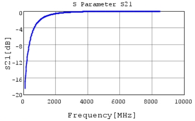
GCQ1555C1H1R9CB01 S21 DCOV, 25degC
