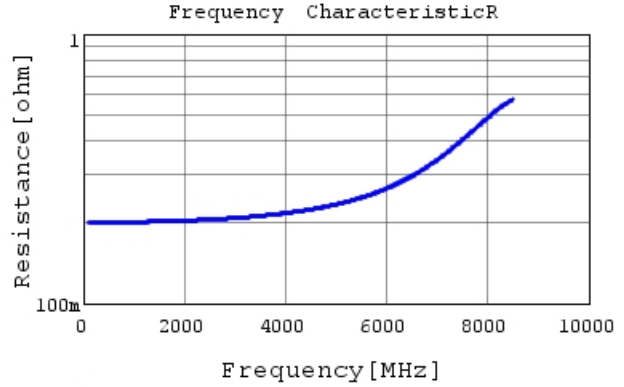
GCQ1555C1H1R9CB01 R DC0V, 25degC
