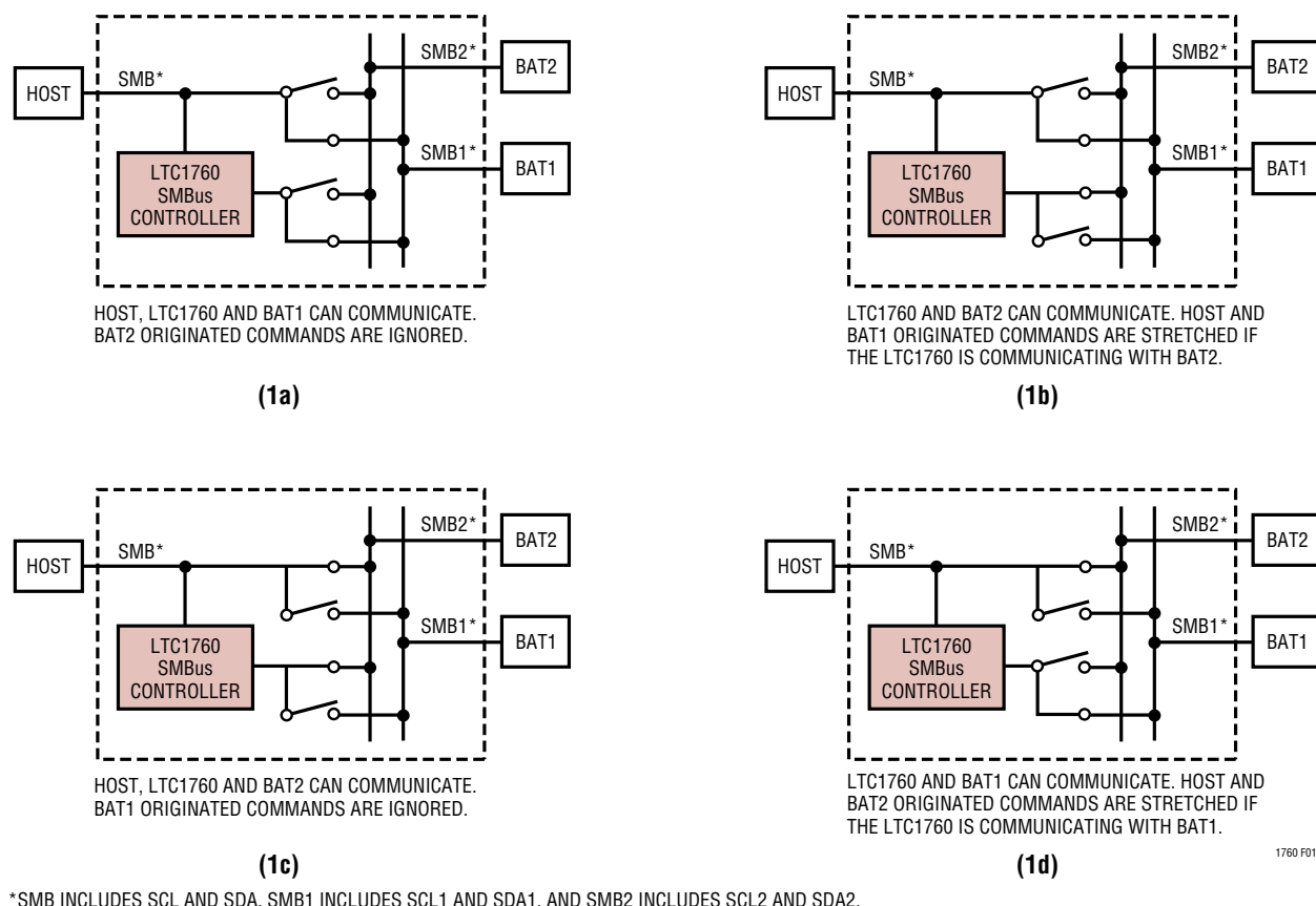
Figure 1. Switch Configurations Used by the LTC1760 for Managing Dual Port Battery Communication
