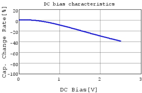
GRM188C80E106ME47 C-DC bias capchange, 25.0c
