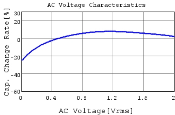
GRM188C80E106ME47 C-AC Voltage capchange, DC
