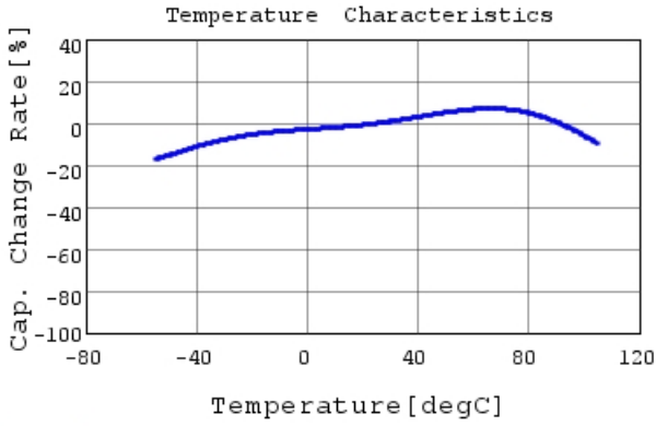
GRM188C80E106ME47 C-Temp. capchange, DC0.0V,
