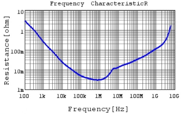
GRM188C80E106ME47 R DCOV, 25degC
