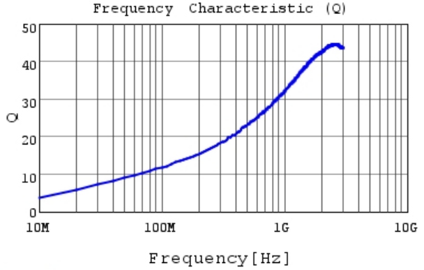
LQG15HZ3N3S02 Q
