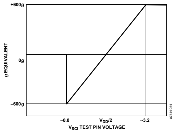
Figure 34. V SCI Signal Chain Input Test Pin Transfer Function
