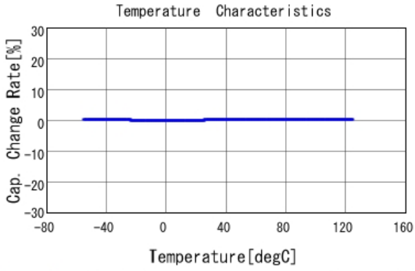
GQM2195C2E1R8BB12 C-Temp. capchange, DCOV, AC1Vrms
