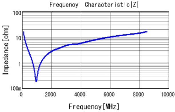
GCM0335C1H101JA16 |Z| DC0V, 25degC
