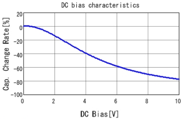
GRT21BC81A106KE01 C-DC bias capchange, 25.0degC, A
