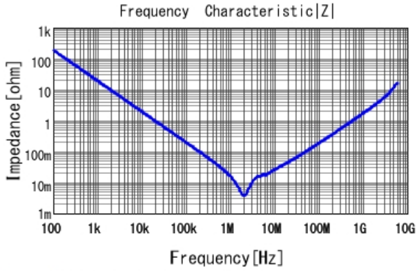
GRT21BC81A106KE01 |Z| DCOV, 25degC
