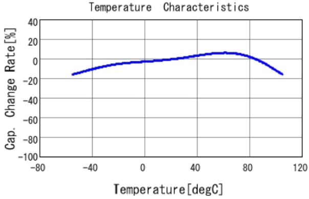
GRT21BC81A106KE01 C-Temp. capchange, DC0.0V, AC0.2
