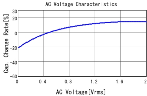
GRT21BC81A106KE01 C-AC Voltage capchange, DCOV, 25
