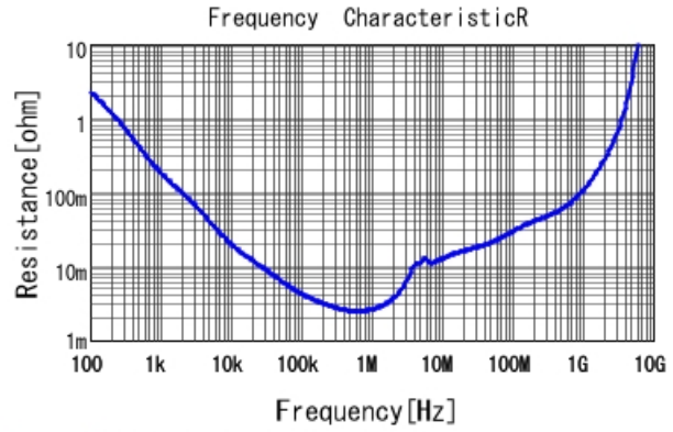
GRT21BC81A106KE01 R DCOV, 25degC
