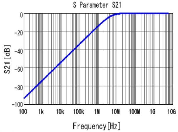
■ GRM033R11C331KA01 S21 DCOV, 20degC
