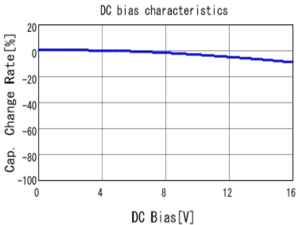
■ GRM033R11C331KA01 C-DC bias capchange, 20.0degC, AC1.
