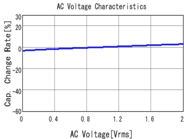
■ GRM033R11C331KA01 C-AC Voltage capchange, DCOV, 20.0d
