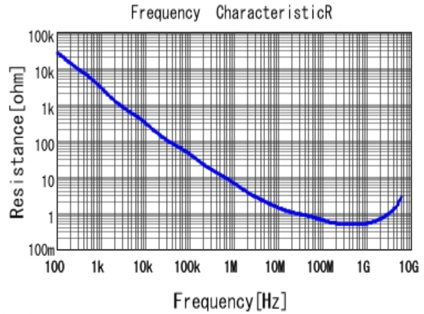
■ GRM033R11C331KA01 R DCOV, 20degC
