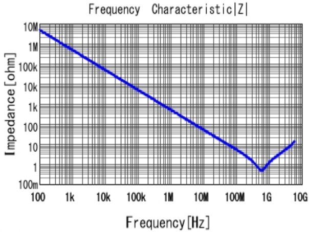
■ GRM033R11C331KA01 |Z| DCOV, 20degC
