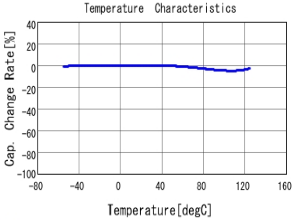
■ GRM033R11C331KA01 C-Temp. capchange, DCO. 0V, AC1.0V rm
