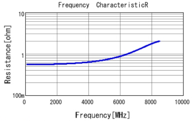
GRM1555C2A1R5CA01 R DCOV, 25degC
