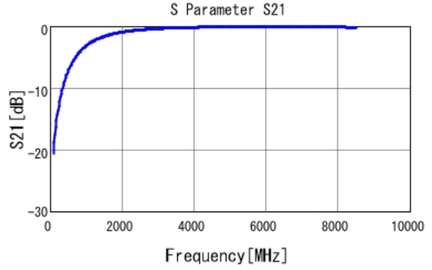
GRM1555C2A1R5CA01 S21 DC0V, 25degC
