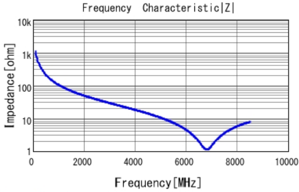
GRM1555C2A1R5CA01 |Z| DCOV, 25degC
