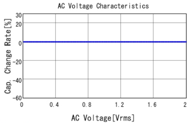
GCM1555G1H101JA16 C-AC Voltage capchange, DCOV, 25
