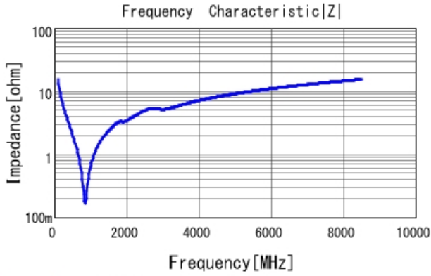
GCM1555G1H101JA16 |Z| DCOV, 25degC
