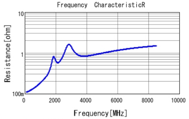
GCM1555G1H101JA16 R DCOV, 25degC
