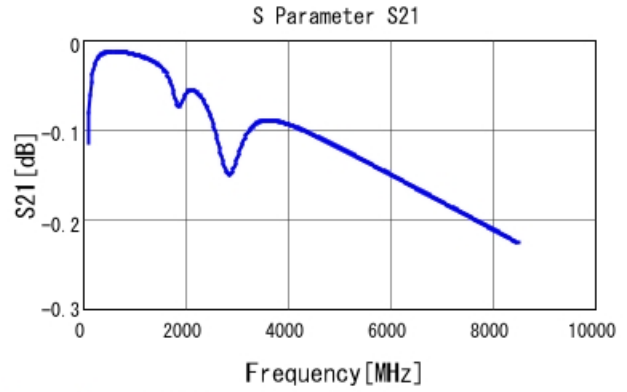
GCM1555G1H101JA16 S21 DCOV, 25degC
