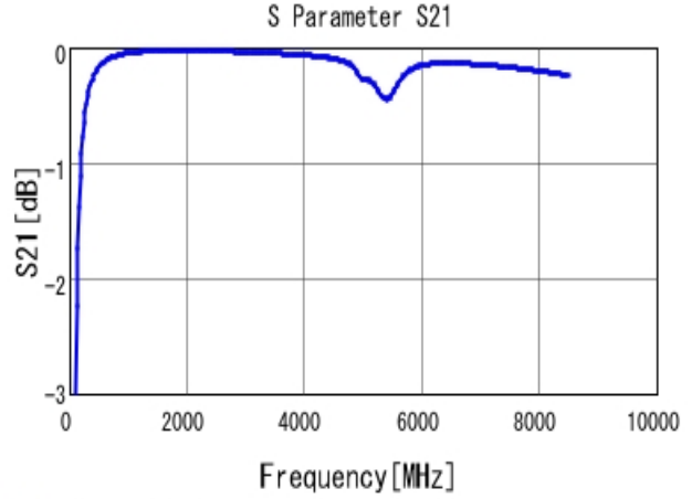
■ GRM0332C1H160JA01 S21 DCOV, 20degC
