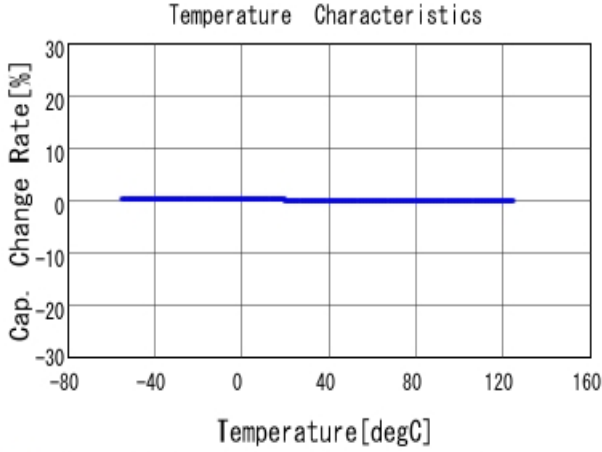
■ GRM0332C1H160JA01 C-Temp. capchange, DCOV, AC1Vrms
