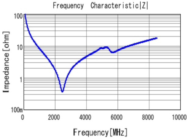
■ GRM0332C1H160JA01 |Z| DCOV, 20degC
