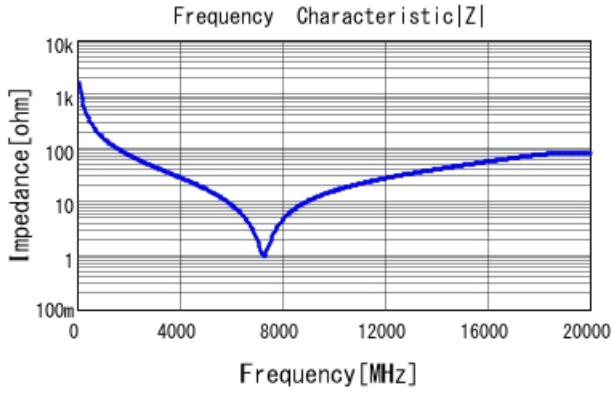
GRM1555C2A1R0CA01 |Z| DCOV, 25degC
