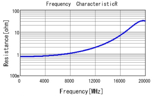
GRM1555C2A1R0CA01 R DCOV, 25degC
