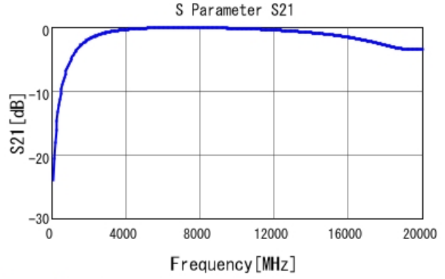
GRM1555C2A1R0CA01 S21 DCOV, 25degC
