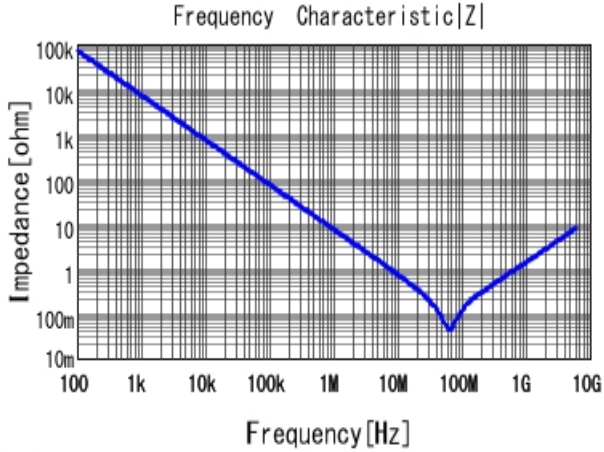
■ GRM033C80G223KE01 |Z| DCOV, 25degC
