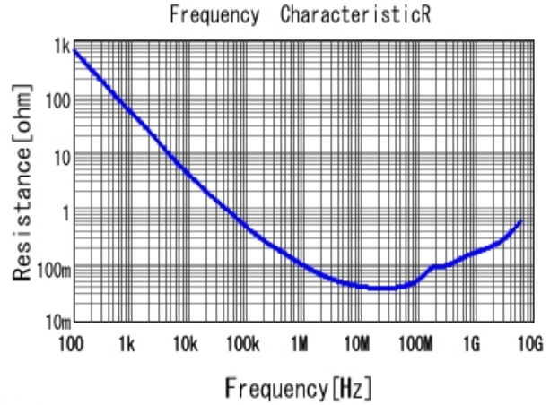
■ GRM033C80G223KE01 R DCOV, 25degC
