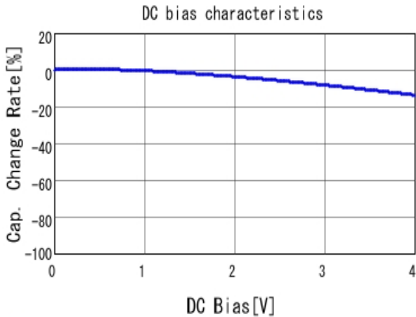
■ GRM033C80G223KE01 C-DC bias capchange, 25.0degC, AC0.
