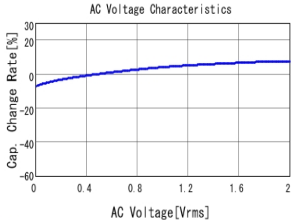
■ GRM033C80G223KE01 C-AC Voltage capchange, DCOV, 25.0d
