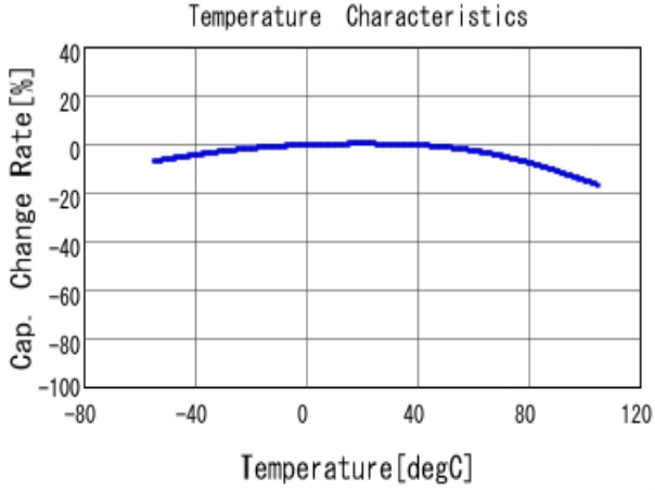
■ GRM033C80G223KE01 C-Temp. capchange, DCO. 0V, ACO. 5Vrm
