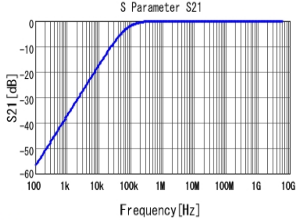
■ GRM033C80G223KE01 S21 DCOV, 25degC
