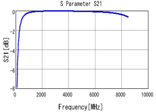
■ GRM0332C1H7R0CA01 S21 DCOV, 20degC
