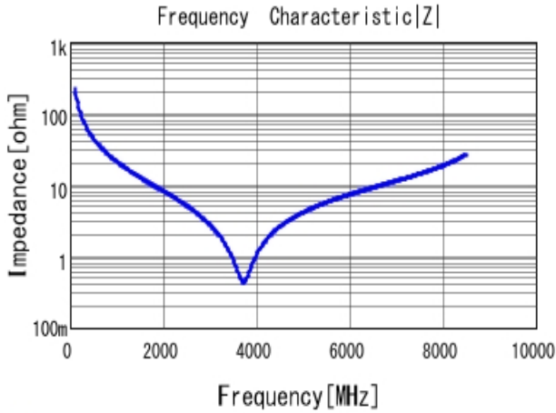
■ GRM0332C1H7R0CA01 |Z| DC0V, 20degC
