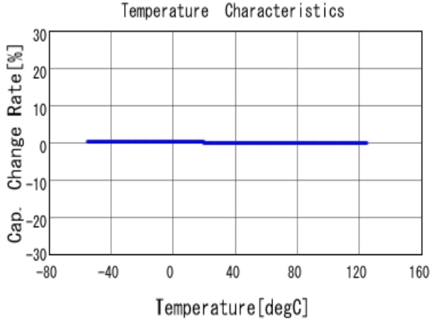
■ GRM0332C1H7R0CA01 C-Temp. capchange, DCOV, AC1Vrms
