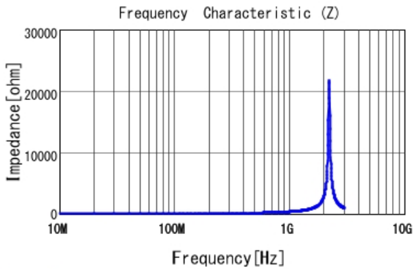
LQP03HQ47NJ02 |Z|
