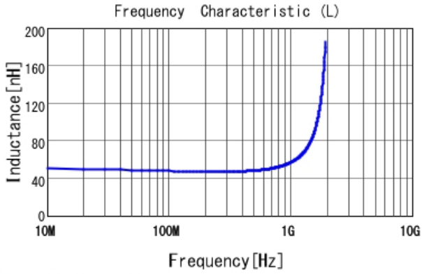
LQP03HQ47NJ02 L
