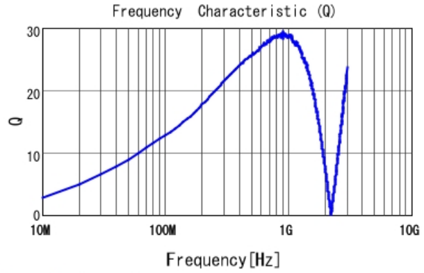
LQP03HQ47NJ02 Q
