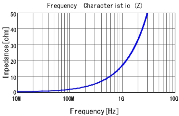
LQP02TQ2N7C02 |Z|
