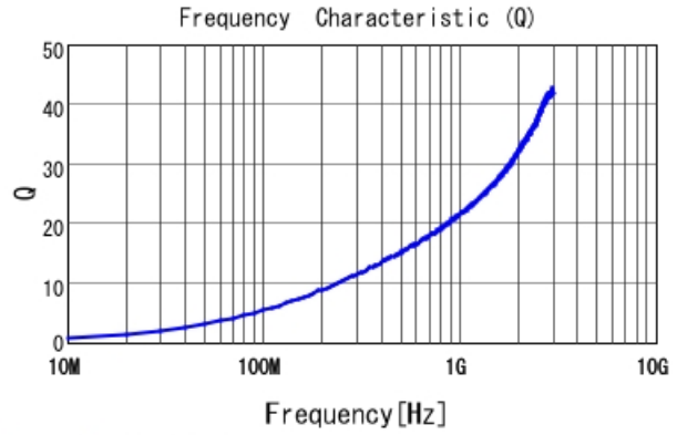
LQP02TQ2N7C02 Q
