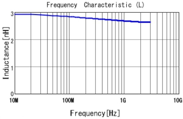
LQP02TQ2N7C02 L
