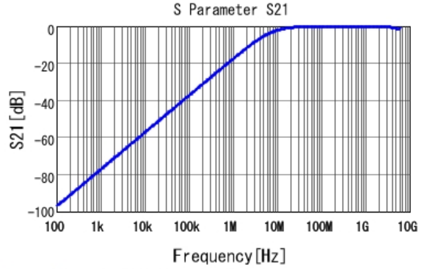
GRM188R71H221KA01 S21 DC0V, 25degC
