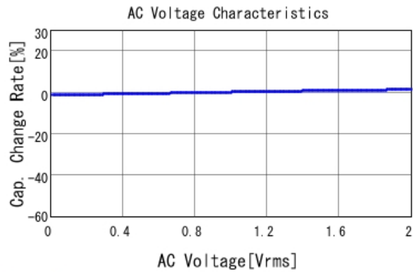
GRM188R71H221KA01 C-AC Voltage capchange, DCOV, 25
