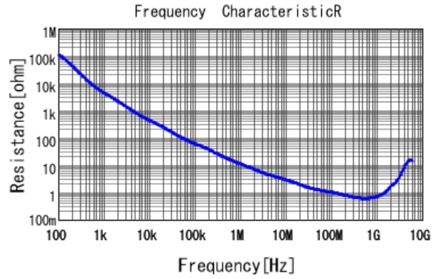
GRM188R71H221KA01 R DCOV, 25degC
