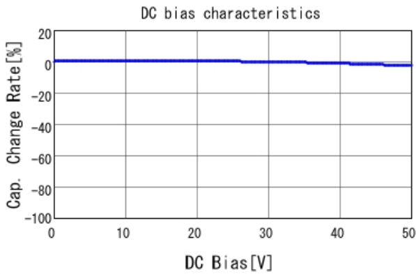
GRM188R71H221KA01 C-DC bias capchange, 25.0degC, A
