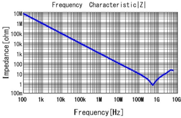
GRM188R71H221KA01 |Z| DCOV, 25degC
