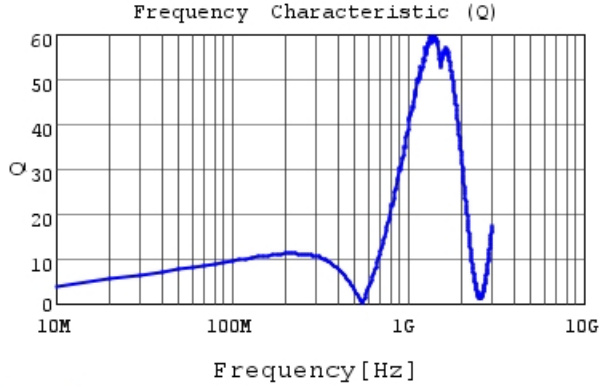
LQG15HSR27G02 Q
