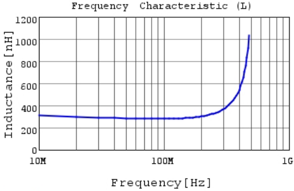
LQG15HSR27G02 L
