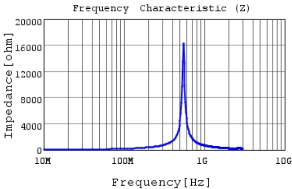
LQG15HSR27G02 |Z|
