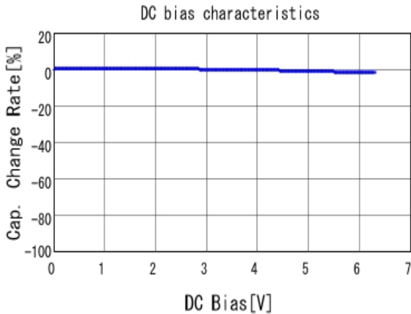
■ GRM033R10J152KA01 C-DC bias capchange, 20.0degC, AC1.
