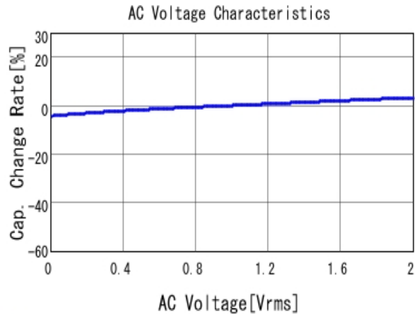
■ GRM033R10J152KA01 C-AC Voltage capchange, DCOV, 20.0d
