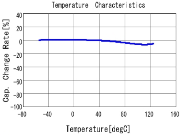
■ GRM033R10J152KA01 C-Temp. capchange, DCO. 0V, AC1. 0Vrm
