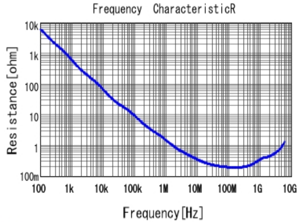
■ GRM033R10J152KA01 R DCOV, 20degC
