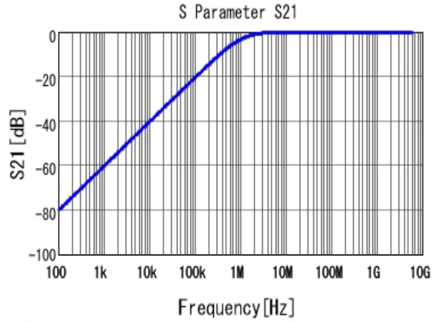
■ GRM033R10J152KA01 S21 DCOV, 20degC
