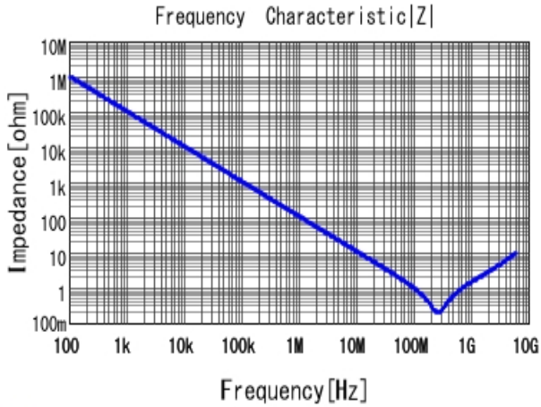
■ GRM033R10J152KA01 |Z| DCOV, 20degC
