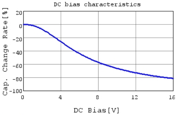
GRM033R61C823KE84 C-DC bias capchange, 25.0c
