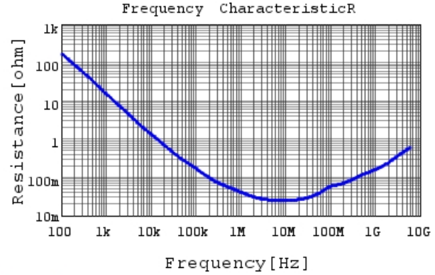
GRM033R61C823KE84 R DC0V, 25degC
