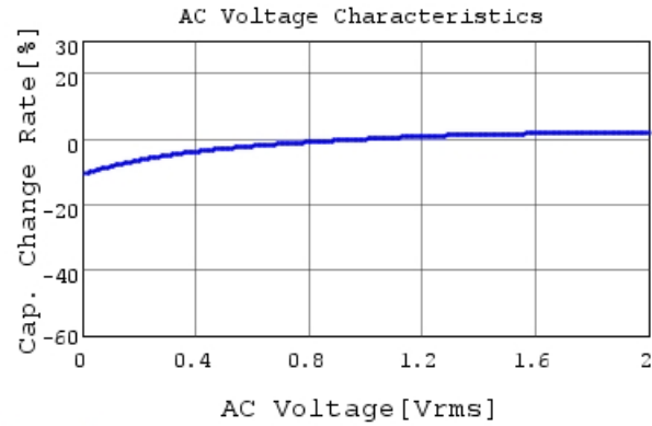
GRM033R61C823KE84 C-AC Voltage capchange, DC
