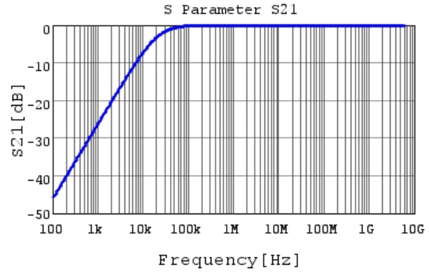
GRM033R61C823KE84 S21 DC0V, 25degC
