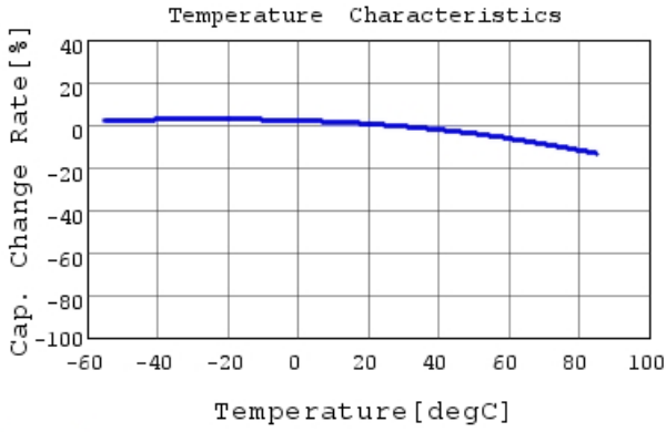
GRM033R61C823KE84 C-Temp. capchange, DC0.0V,
