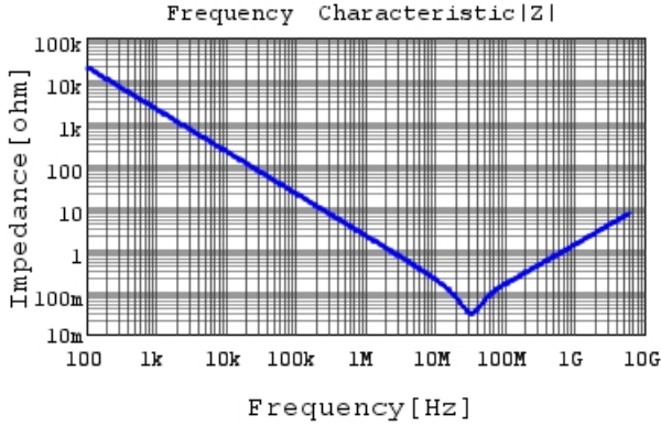
GRM033R61C823KE84 |Z| DC0V, 25degC
