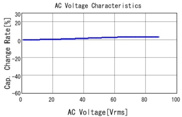
GCJ31CR72E333KXJ3 C-AC Voltage capchange, DCOV, 25
