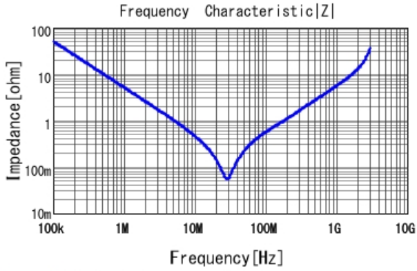
GCJ31CR72E333KXJ3 |Z| DCOV, 25degC
