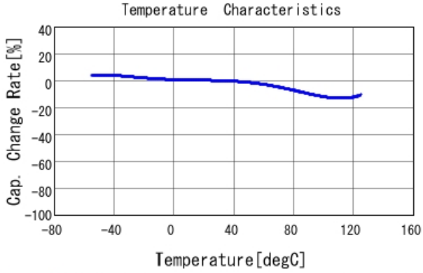
GCJ31CR72E333KXJ3 C-Temp. capchange, DCOV, AC1Vrms
