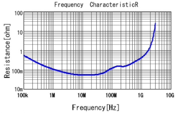
GCJ31CR72E333KXJ3 R DCOV, 25degC
