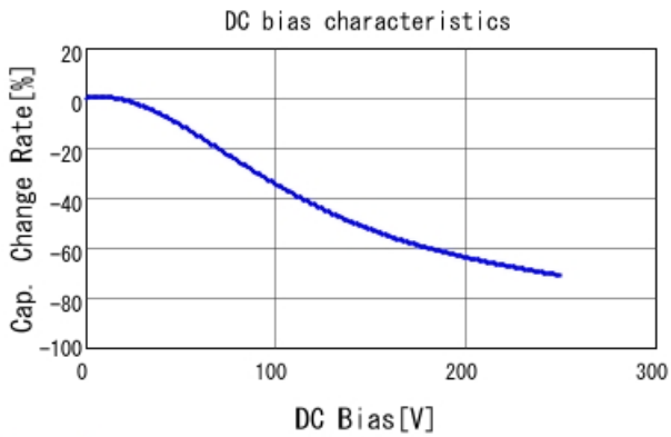
GCJ31CR72E333KXJ3 C-DC bias capchange, 25.0degC, A
