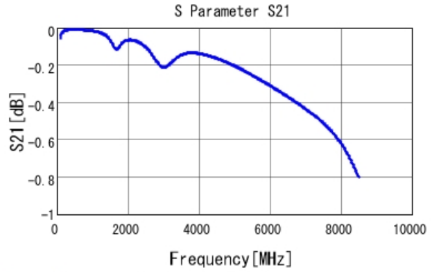
GRM2165C2A151JA01 S21 DCOV, 25degC
