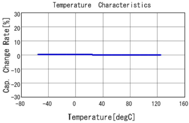
GRM2165C2A151JA01 C-Temp. capchange, DCOV, AC1Vrms
