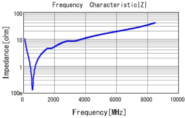
GRM2165C2A151JA01 |Z| DCOV, 25degC
