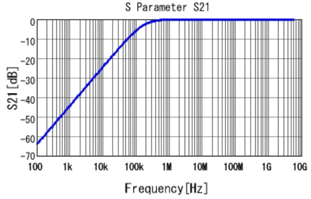
■ GRM033B11A103MA01 S21 DCOV, 20degC
