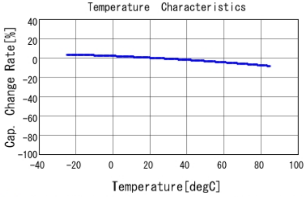
■ GRM033B11A103MA01 C-Temp. capchange, DCO. 0V, AC1. 0Vrm
