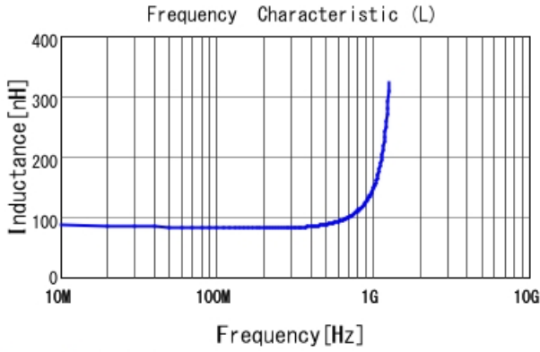
LQP03TN82NHZ2 L
