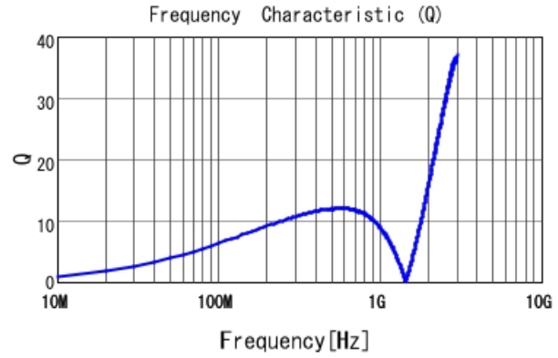
LQP03TN82NHZ2 Q
